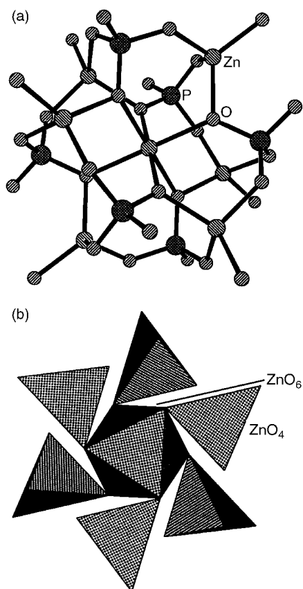
Fig. 7 (a) Ball and stick diagram showing the basic building unit in IV . (b) The unique \text{Zn}_7\text{O}_6 cluster in a tooth-wheel arrangement.
