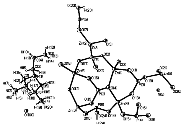
Fig. 3 ORTEP plot of the layered zinc phosphate, III , [\text{C}_6\text{N}_4\text{H}_{21}][\text{NH}_4][\text{Zn}_6(\text{PO}_4)_4(\text{HPO}_4)_2] \cdot \text{H}_2\text{O} .
